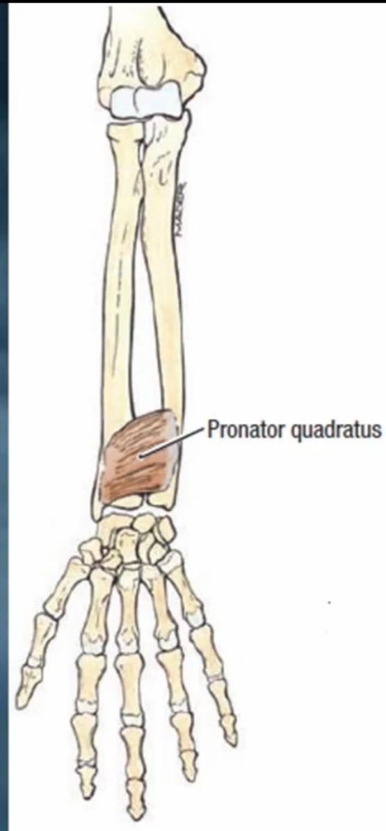
4th layer
