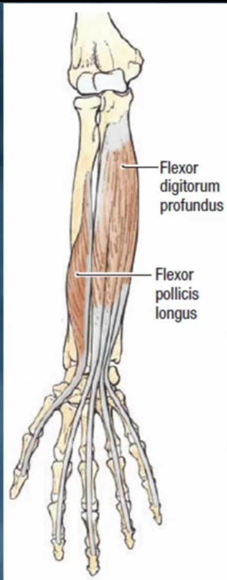
3rd layer
